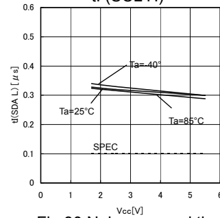
Fig.30 Noise removal time t(SDA L)
