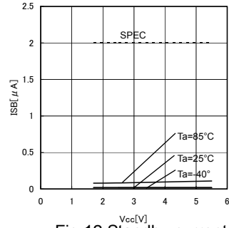
Fig.12 Standby current Isub
