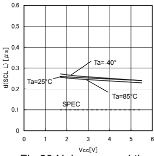
Fig.28 Noise removal time t(SCL L)
