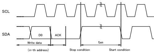
Fig.1-(c) Write cycle timing
