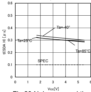
Fig.29 Noise removal time t(SDA H)
