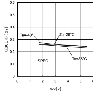
Fig.27 Noise removal time t(SCL H)
